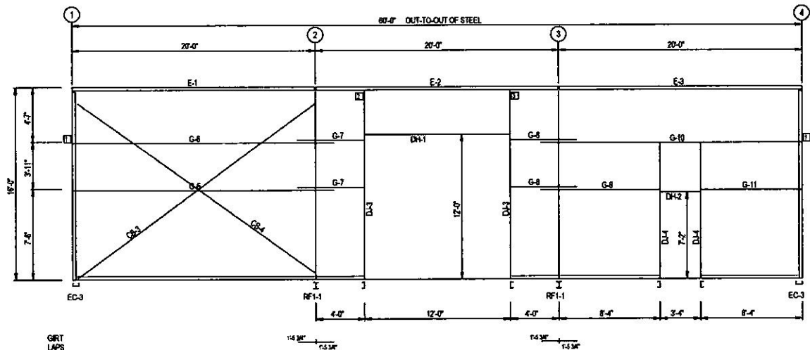
SIDEWALL FRAMING: FRAME LINE A
